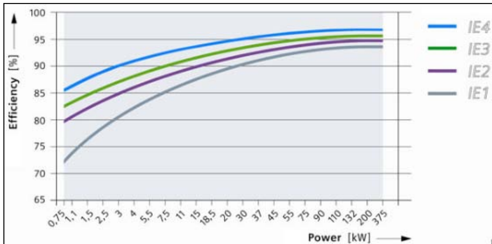
Figure 7.1: Efficiency classes IE1 to IE4 Source: IEC 60034-30-1
