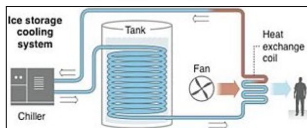
Figure 8.17: Ice-Bank System
