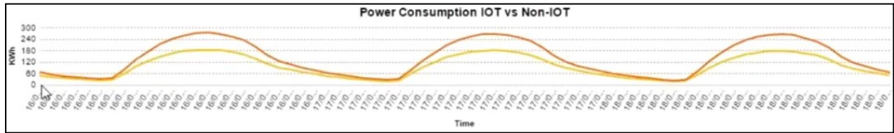
Figure 7.9: Compressor Power Consumption – IOT vs Non-IOT
