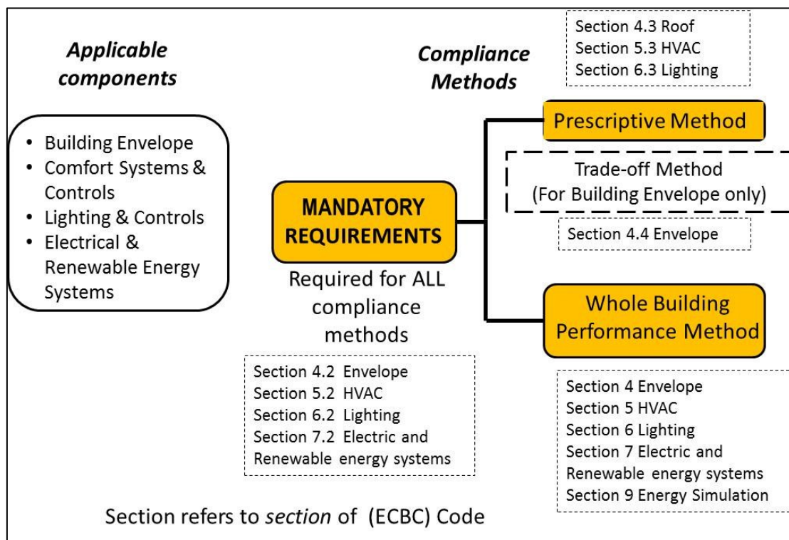
Figure 3.5: ECBC-Compliance Approach
