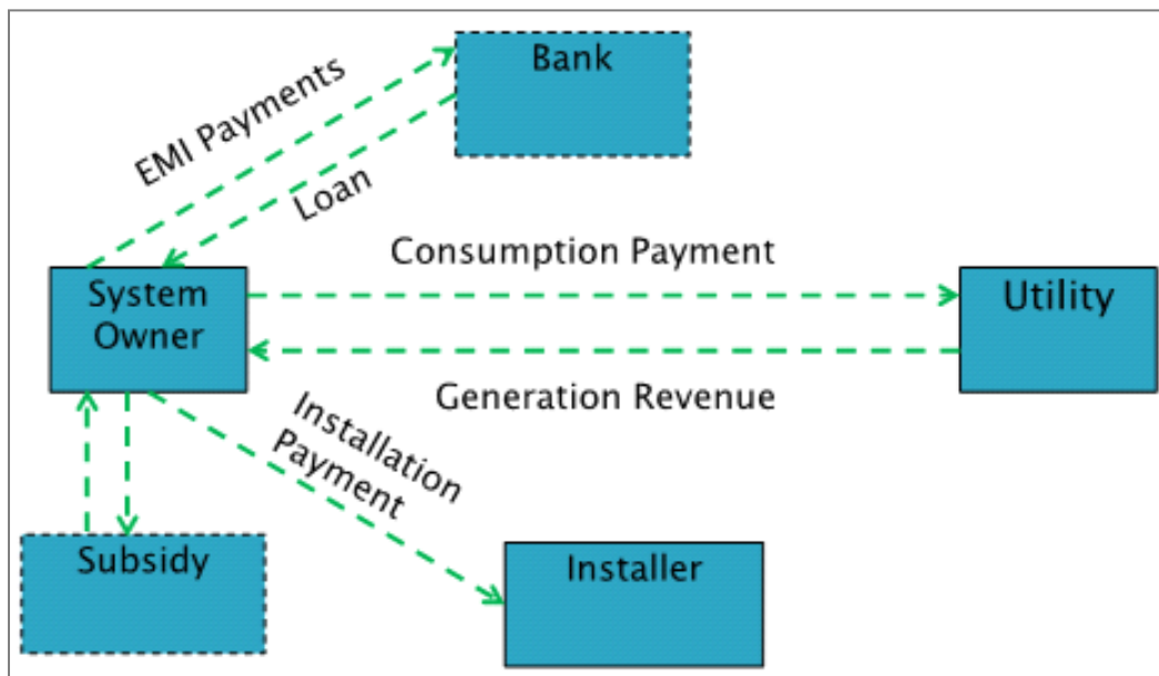
Figure 9.15: CAPEX Model
