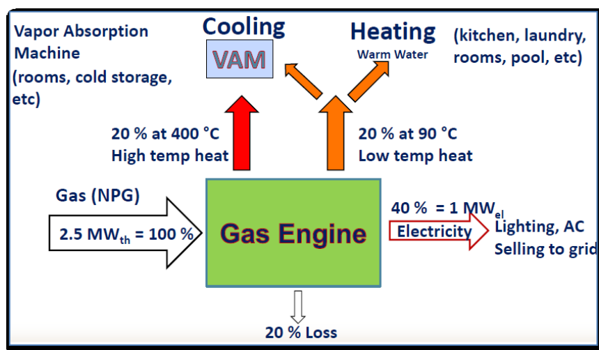
Figure 7.18: Trigeneration Application
