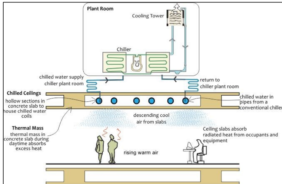
Figure: 8.19: Schematic Diagram of a Radiant Cooling System.
