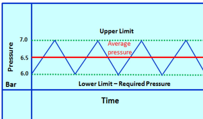
Figure 7.7: VFD Control
