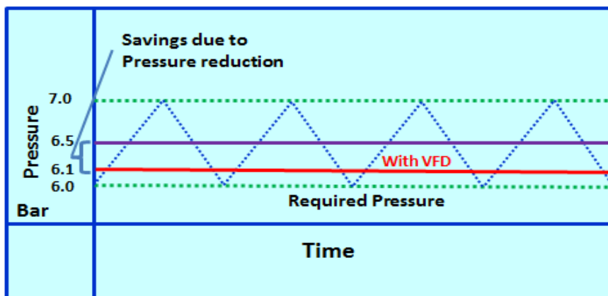
Figure 7.6: Load/Unload Control
