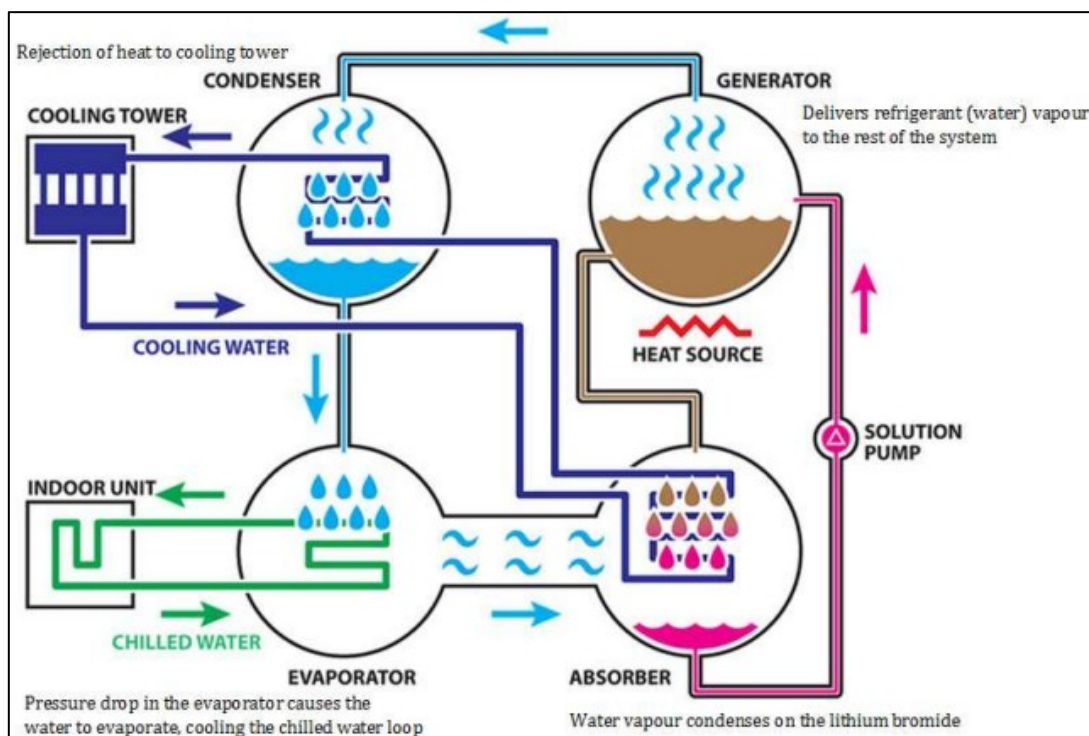
Figure 7.17: Trigereneration
